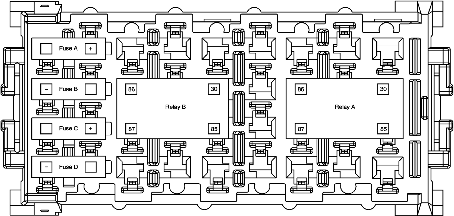
Fuse Block - Mobile Radio, Device Usage (9L4)
